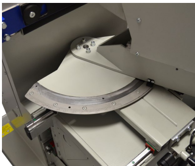
Bohraggregat schwenkbar - 65° - 0 - 65°
